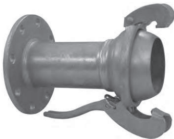
Type B male with 150 ASA flange
